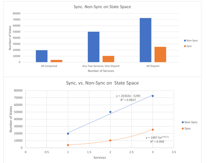
Fig. 8. Bar Graph and Line Graph Representations of Synchronous Firing with Comprehensive Services on State Space
