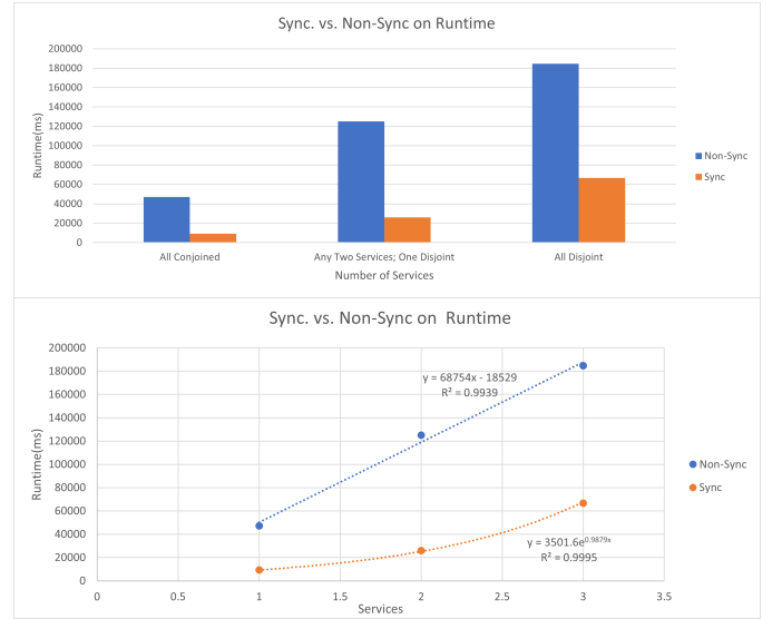
Fig. 7. Bar Graph and Line Graph Representations of Synchronous Firing with Comprehensive Services on Runtime
