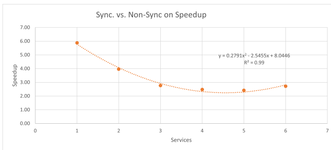
Fig. 6. Speedup (Amdahl's) Obtained When Using Synchronous Firing
