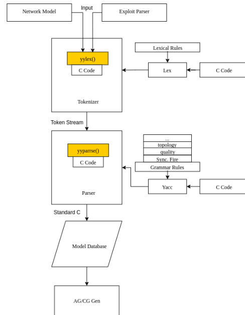
Fig. 2. Inclusion of Synchronous Firing into GNU Bison, GNU Flex, and the overall program
