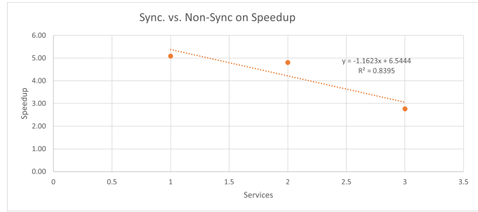
Fig. 9. Speedup (Amdahl's) Obtained When Using Synchronous Firing with Comprehensive Services
