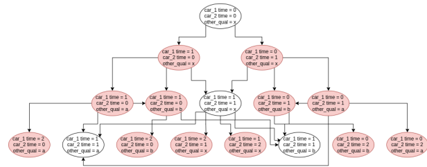
Fig. 1. A network without Synchronous Firing generating infeasible states
