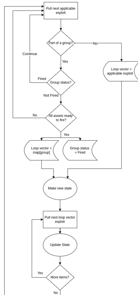
Fig. 3. Synchronous Firing in the Graph Generation Process
