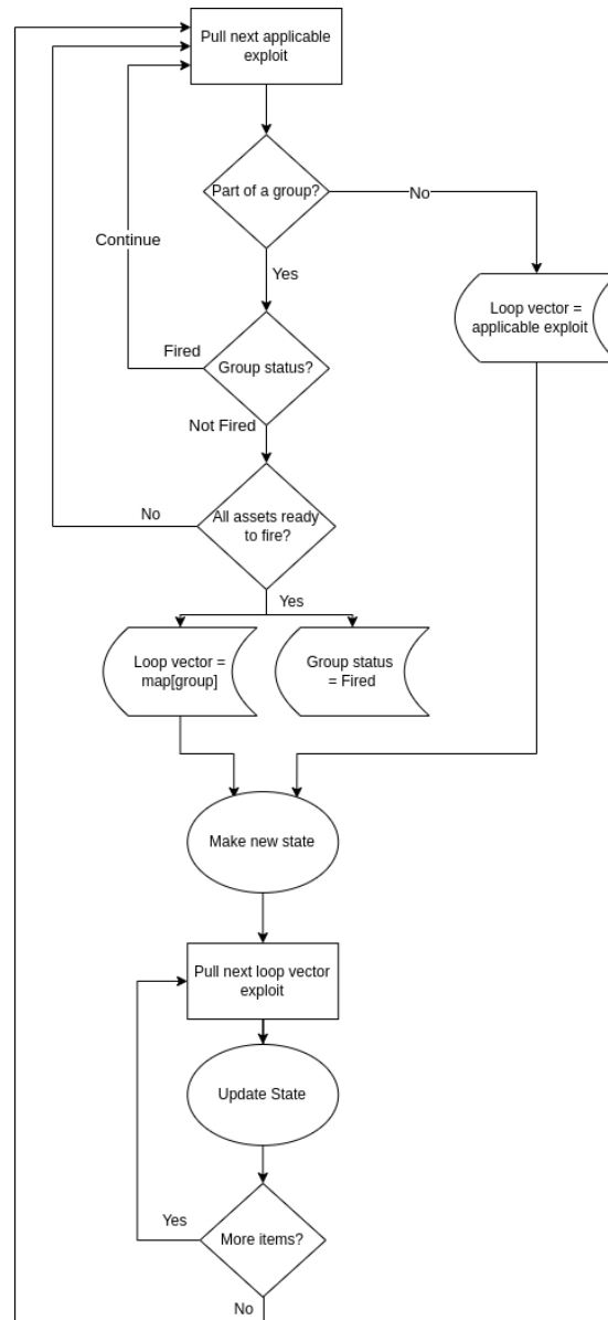
Synchronous Firing in the Graph Generation Process
