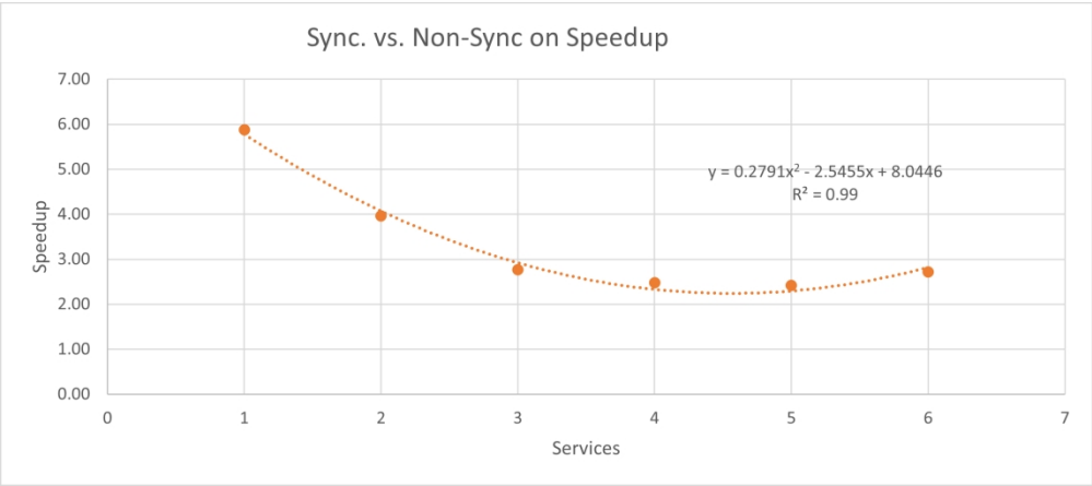
Speedup (Amdahl's) Obtained When Using Synchronous Firing 475x210mm (130 x 130 DPI)
