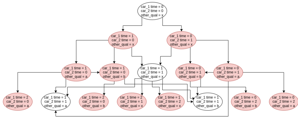
A network without Synchronous Firing generating infeasible states
