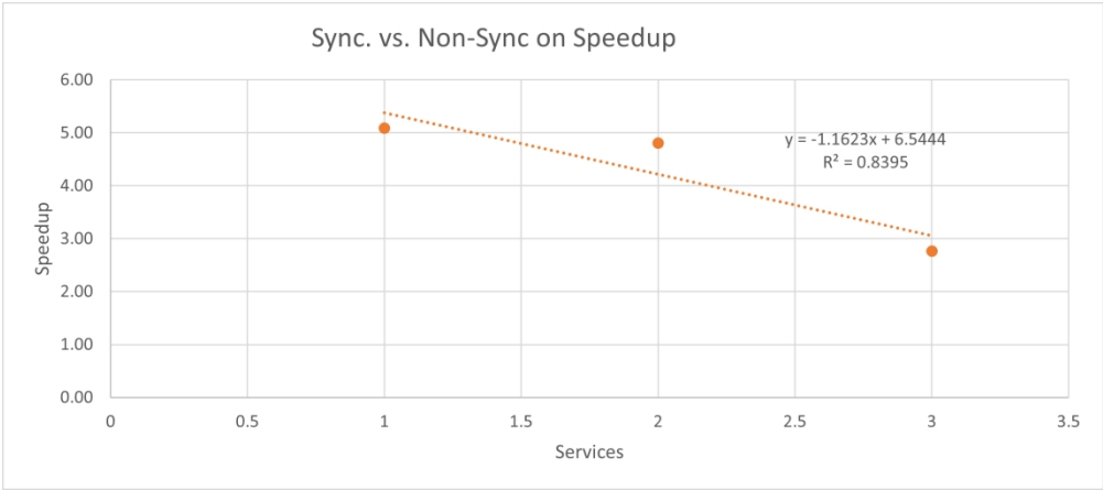
Speedup (Amdahl's) Obtained When Using Synchronous Firing with Comprehensive Services 475x210mm (130 x 130 DPI)
