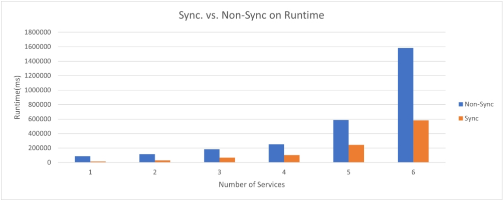
Bar Graph and Line Graph Representations of Synchronous Firing on Runtime 537x212mm (130 x 130 DPI)
