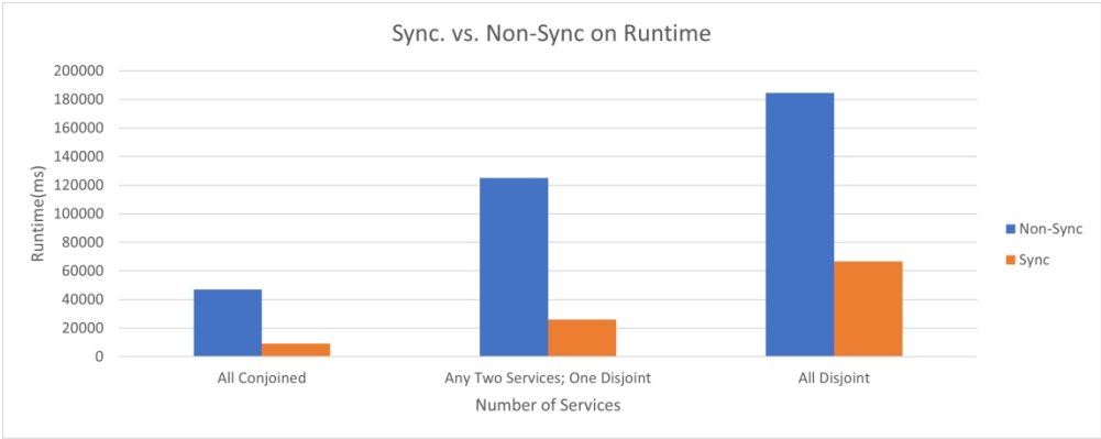
Bar Graph and Line Graph Representations of Synchronous Firing with Comprehensive Services on Runtime 537x212mm (130 x 130 DPI)
