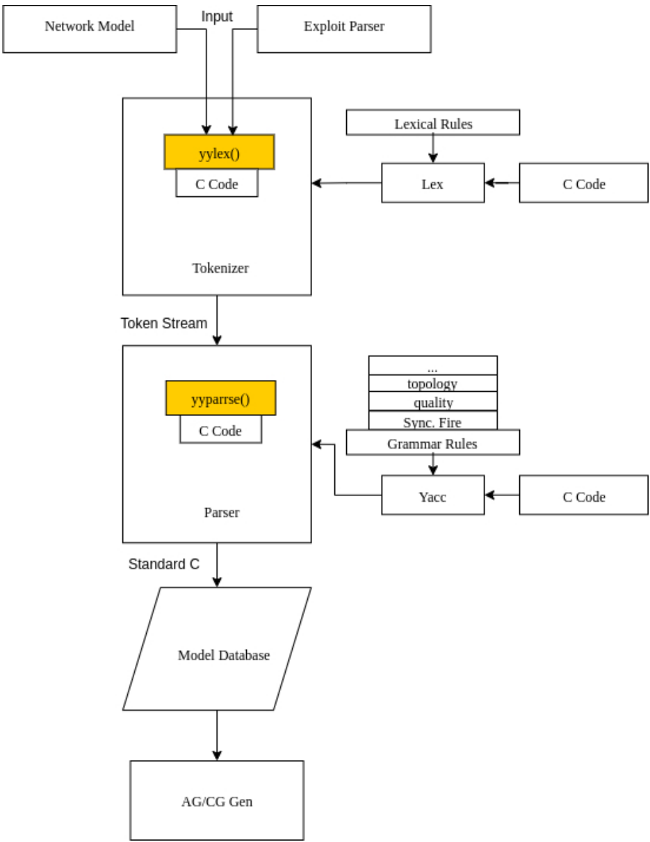
Inclusion of Synchronous Firing into GNU Bison, GNU Flex, and the overall program 193x249mm (72 x 72 DPI)
