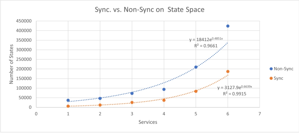
Bar Graph and Line Graph Representations of Synchronous Firing on State Space 475x211mm (130 x 130 DPI)
