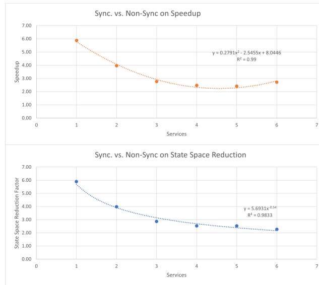
FIGURE 7. Speedup (Amdahl's) and State Space Reduction Factor Obtained When Using Synchronous Firing
