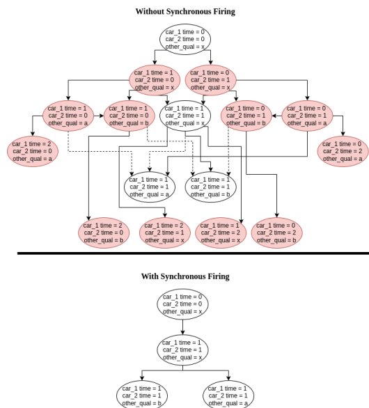
FIGURE 4. Car Example With and Without Synchronous Firing
