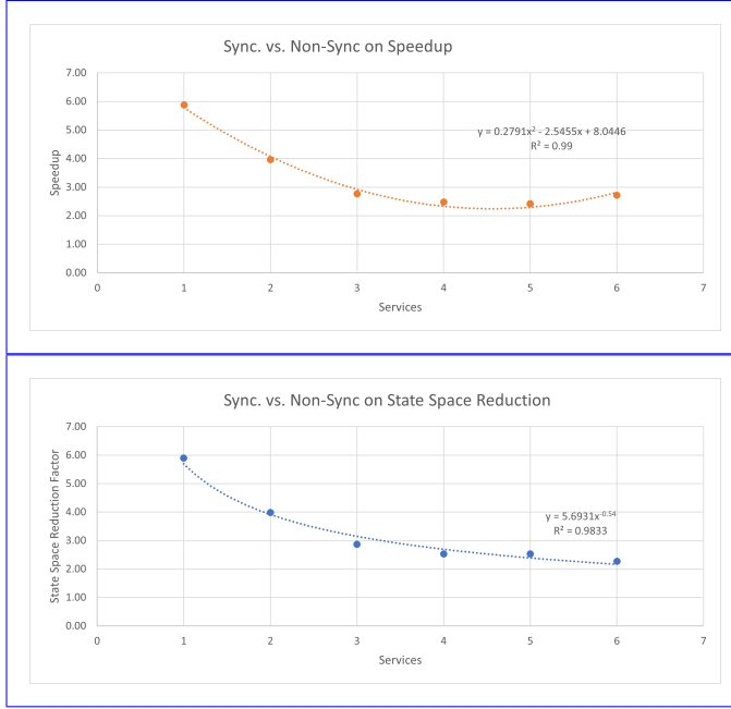
FIGURE 7. Speedup (Amdahl's) and State Space Reduction Factor Obtained When Using Synchronous Firing
