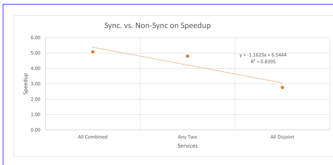
FIGURE 10. Speedup (Amdahl's) Obtained When Using Synchronous Firing with Comprehensive Services
