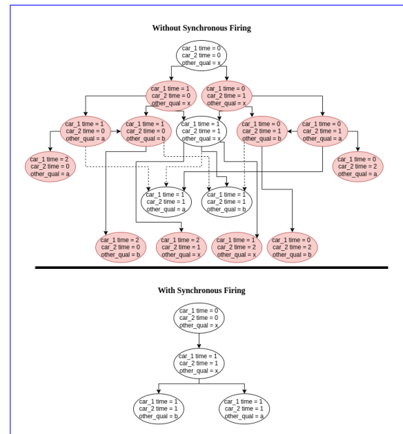
FIGURE 4. Car Example With and Without Synchronous Firing
