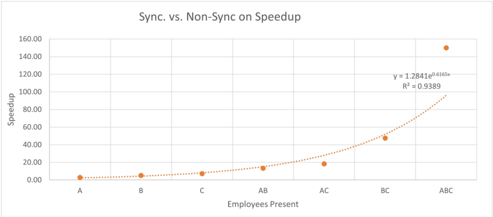
Speedup (Amdahl's) and State Space Reduction Factor Obtained When Using Synchronous Firing 478x210mm (130 x 130 DPI)
