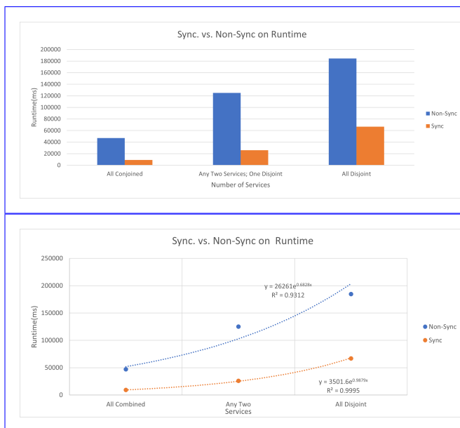
FIGURE 8. Bar Graph and Line Graph Representations of Synchronous Firing with Comprehensive Services on Runtime
