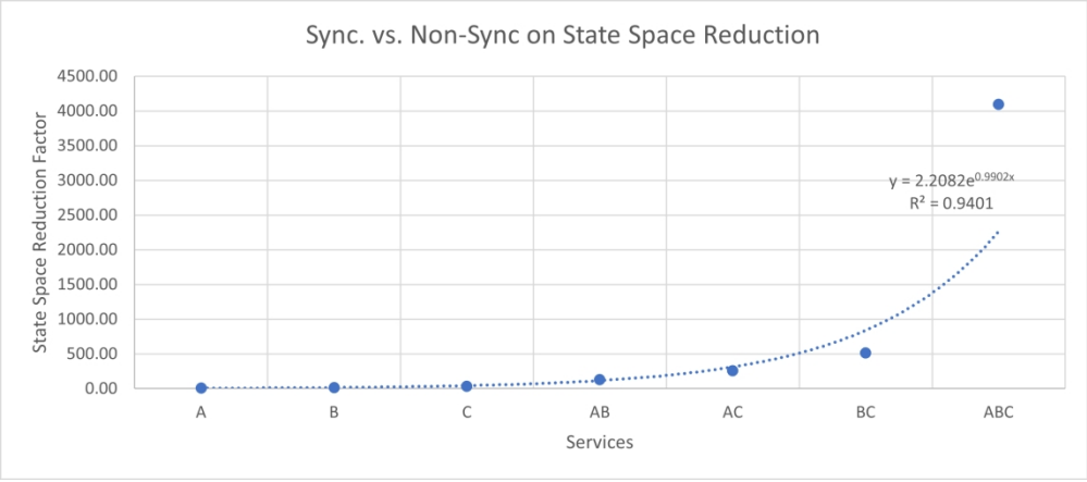
21 Speedup (Amdahl's) and State Space Reduction Factor Obtained When Using Synchronous Firing 22 23 478x210mm (130 x 130 DPI) 24 25 26 27 28 29 30 31 32 33 34 35 36 37 38 39 40 41 42 43 44 45 46 47 48 49 50 51 52 53 54 55 56 57 58 59 60
