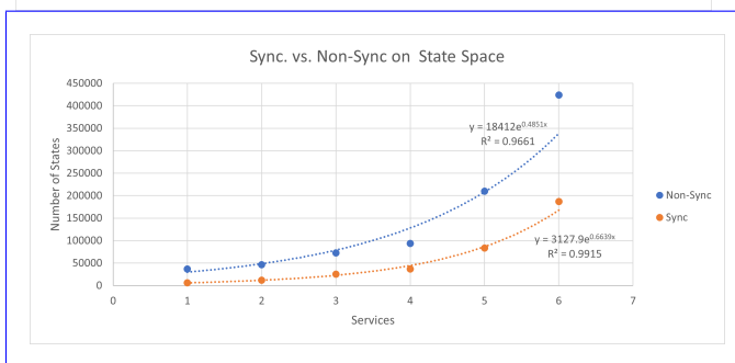
FIGURE 6. Bar Graph and Line Graph Representations of Synchronous Firing on State Space
