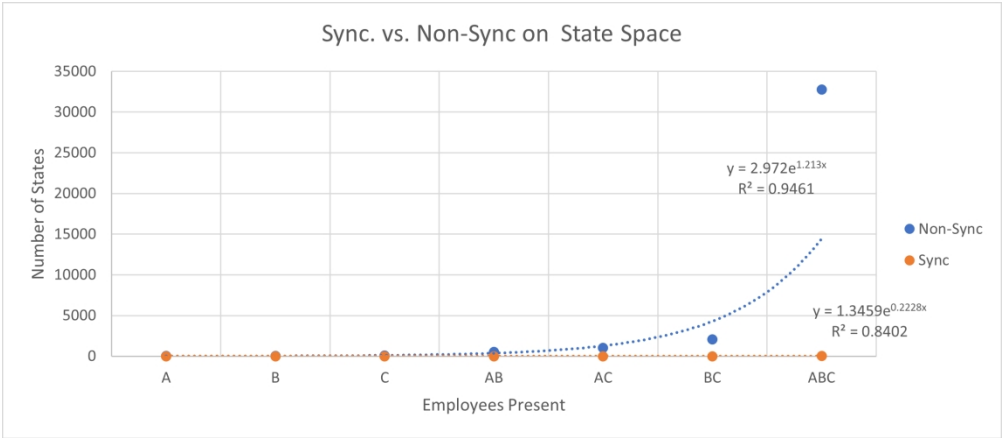
Synchronous Firing on State Space and Runtime for the DMCA Takedown Environment 483x211mm (130 x 130 DPI)
