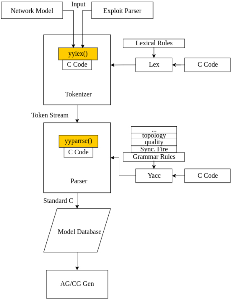
Inclusion of Synchronous Firing into GNU Bison, GNU Flex, and the overall program
