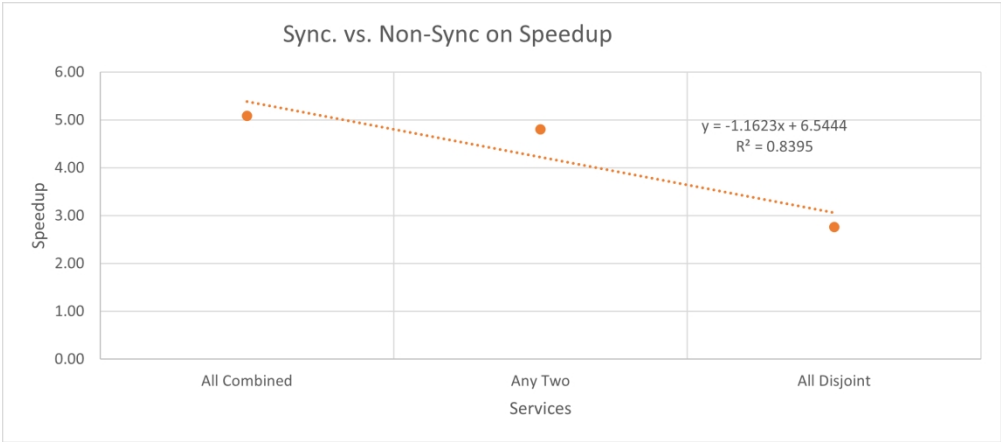
Speedup (Amdahl's) Obtained When Using Synchronous Firing with Comprehensive Service 478x210mm (130 x 130 DPI)
