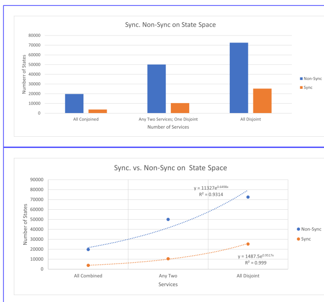
FIGURE 9. Bar Graph and Line Graph Representations of Synchronous Firing with Comprehensive Services on State Space
