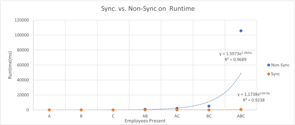
Synchronous Firing on State Space and Runtime for the DMCA Takedown Environment 499x210mm (130 x 130 DPI)
