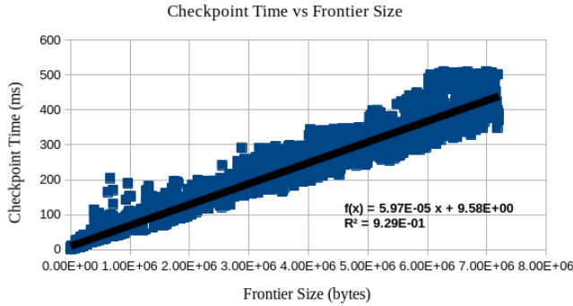
Fig. 3. Time Taken to Checkpoint as the Size of the Frontier Grows
