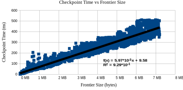
Fig. 4. Time Taken to Checkpoint as the Size of the Frontier Grows
