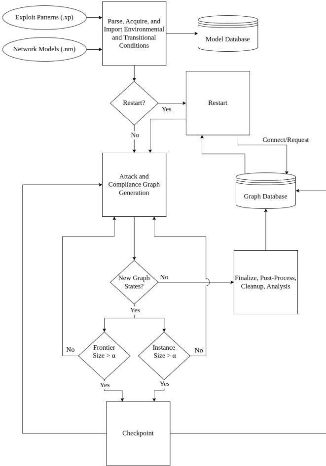
Fig. 1. Program Flow of the Attack and Compliance Graph Generation Process with C/R
