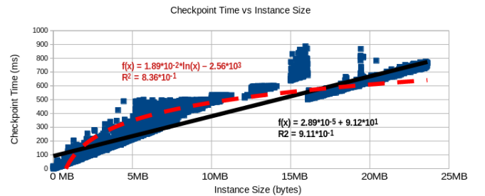
Fig. 3. Time Taken to Checkpoint as the Size of the Instance Grows
