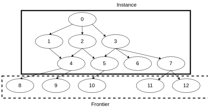
Fig. 2. An Attack or Compliance Graph Undergoing Generation
