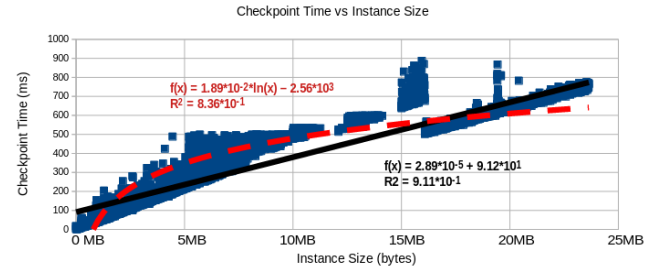
FIGURE 2. Time Taken to Checkpoint as the Size of the Instance Grows
