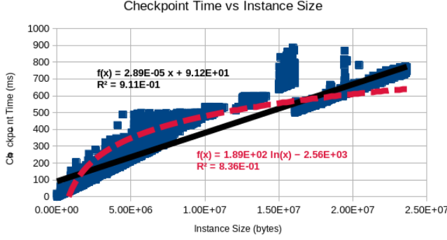
Fig. 2. Time Taken to Checkpoint as the Size of the Instance Grows
