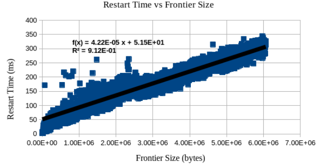
Fig. 4. Time Taken to Restart as the Size of the Frontier Grows
