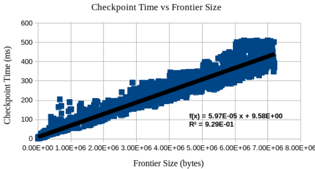
Fig. 3. Time Taken to Checkpoint as the Size of the Frontier Grows
