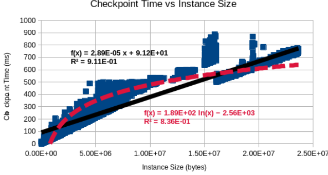
Fig. 2. Time Taken to Checkpoint as the Size of the Instance Grows
