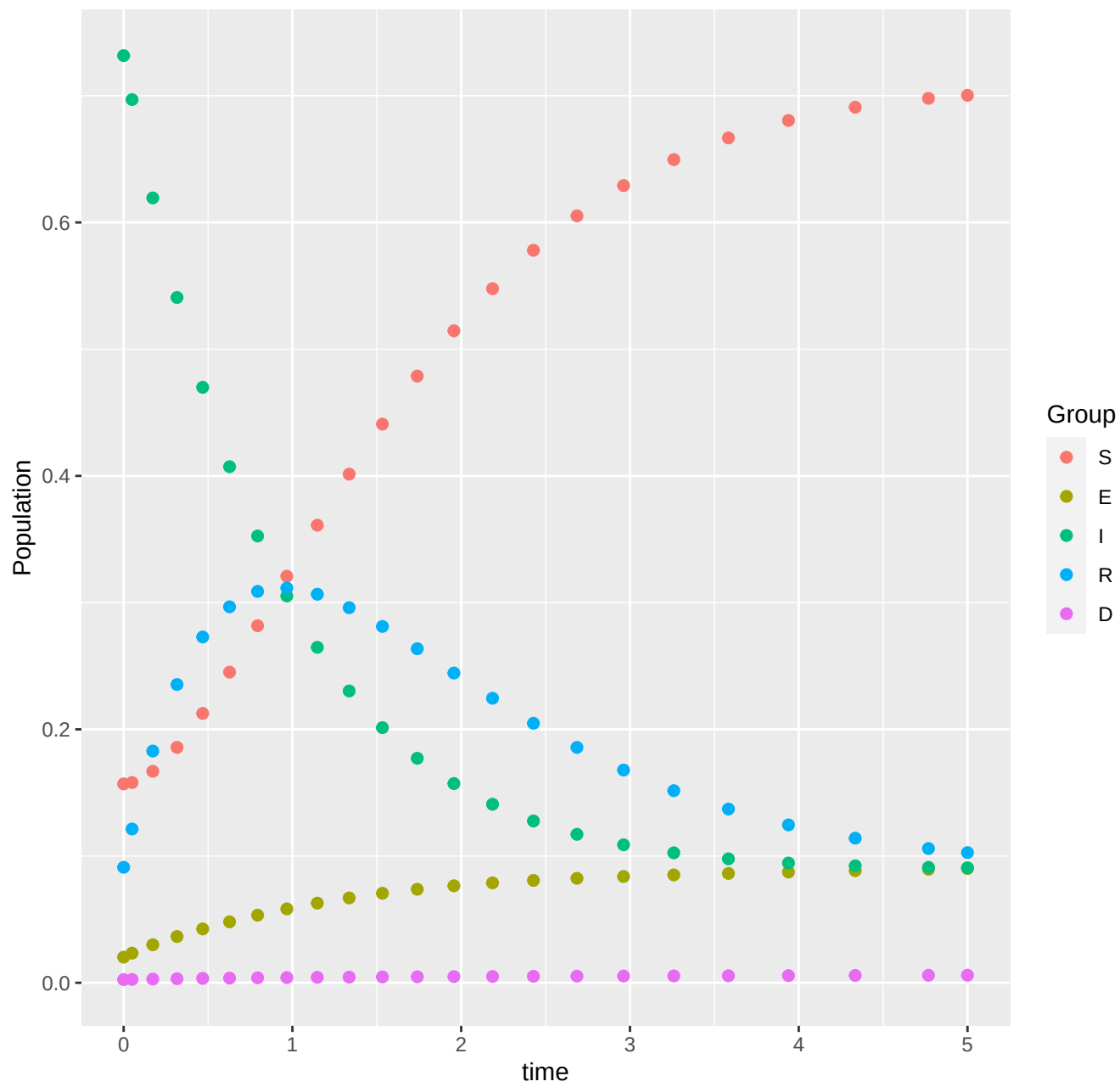
SEIRDS Model Using ODE45
