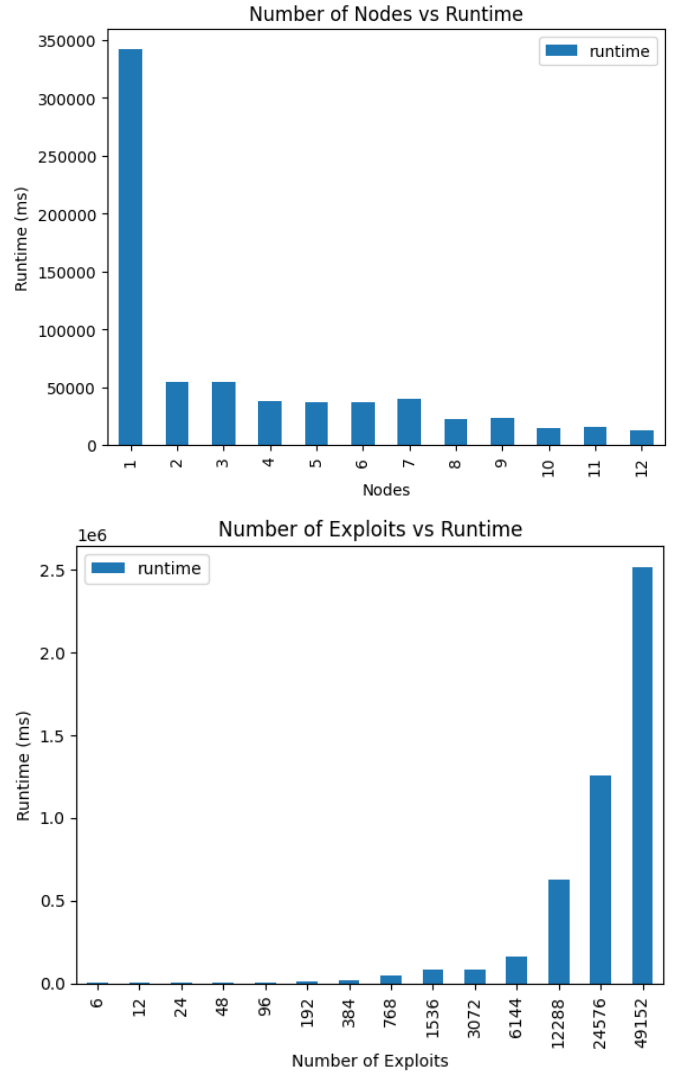
Fig. 9. Number of Nodes and Exploits (Averaged) vs. Runtime (ms)
