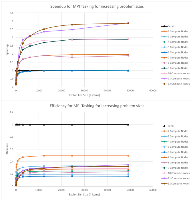
Fig. 8. Speedup and Efficiency of the MPI Tasking Approach for a Varying Number of Compute Nodes with an Increasing Problem Size
