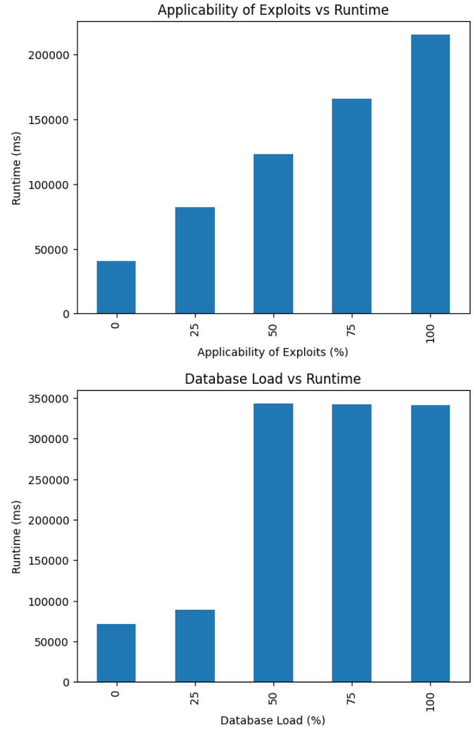
Fig. 10. Applicability of Exploits (%) and Database Load (%) (Averaged) vs. Runtime (ms)
