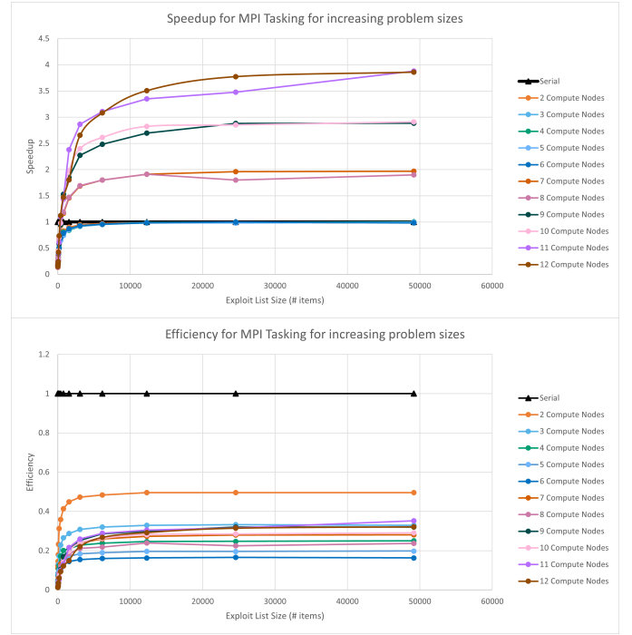
Fig. 9. Speedup and Efficiency of the MPI Tasking Approach for a Varying Number of Compute Nodes with an Increasing Problem Size
