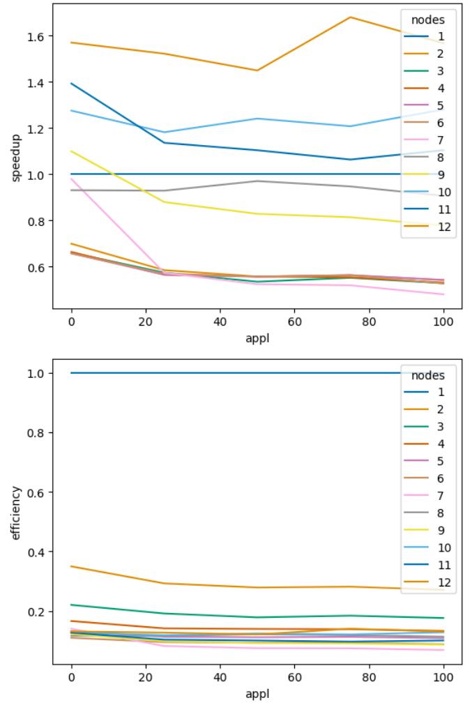
Fig. 15. Mean Speedup and Efficiency for the Applicability of Exploit Parameter Across the Number of Compute Nodes
