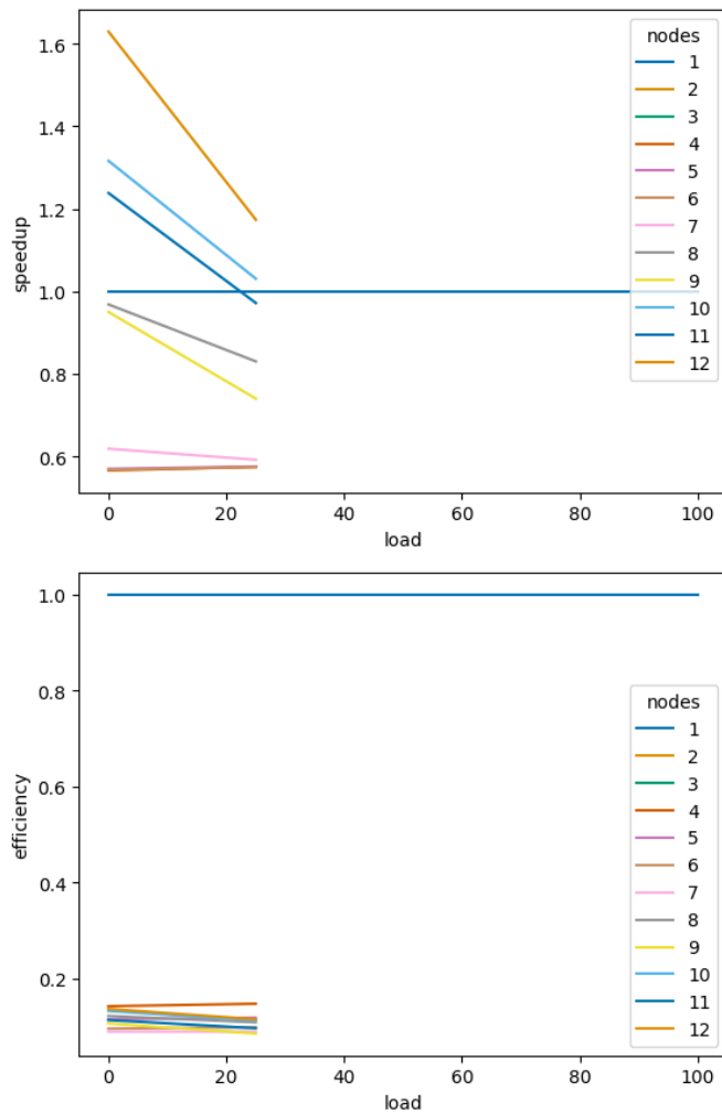
Fig. 16. Mean Speedup and Efficiency for the Database Load Parameter Across the Number of Compute Nodes
