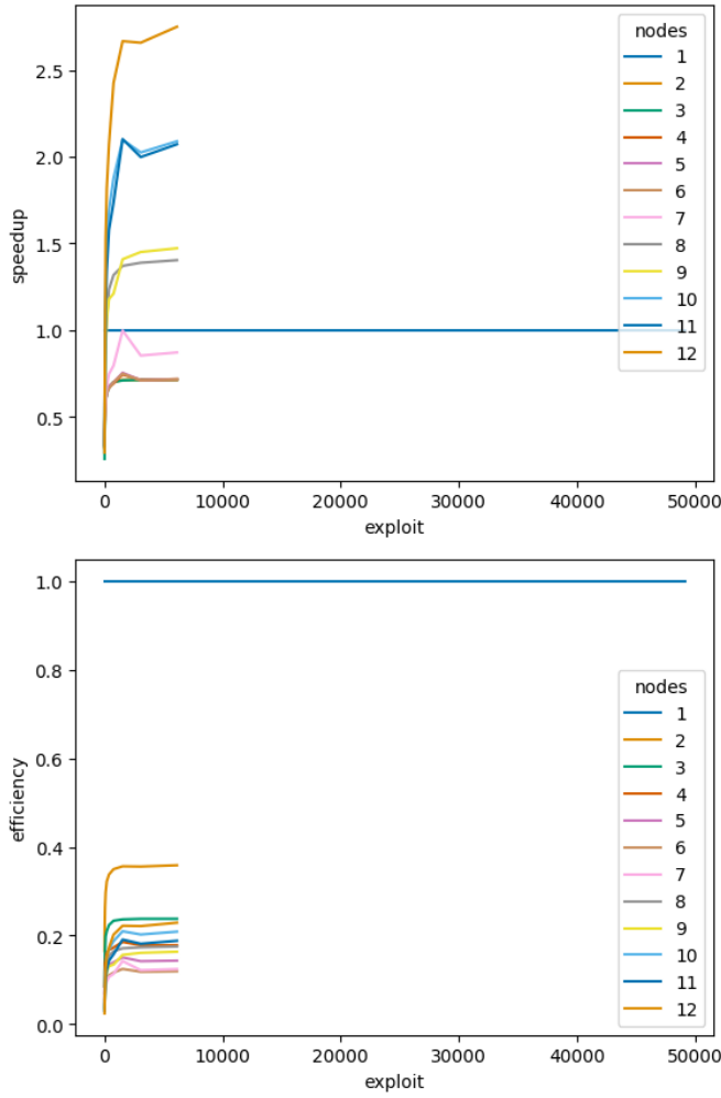
Fig. 14. Mean Speedup and Efficiency for the Exploit Parameter Across the Number of Compute Nodes
