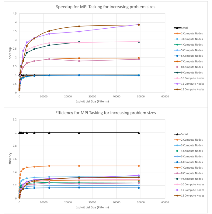
Fig. 8. Speedup and Efficiency of the MPI Tasking Approach for a Varying Number of Compute Nodes with an Increasing Problem Size
