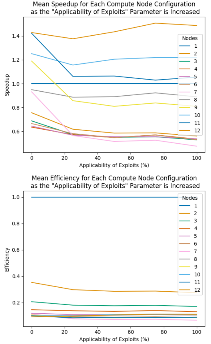
Fig. 14. Mean Speedup and Efficiency for the Applicability of Exploit Parameter Across the Number of Compute Nodes
