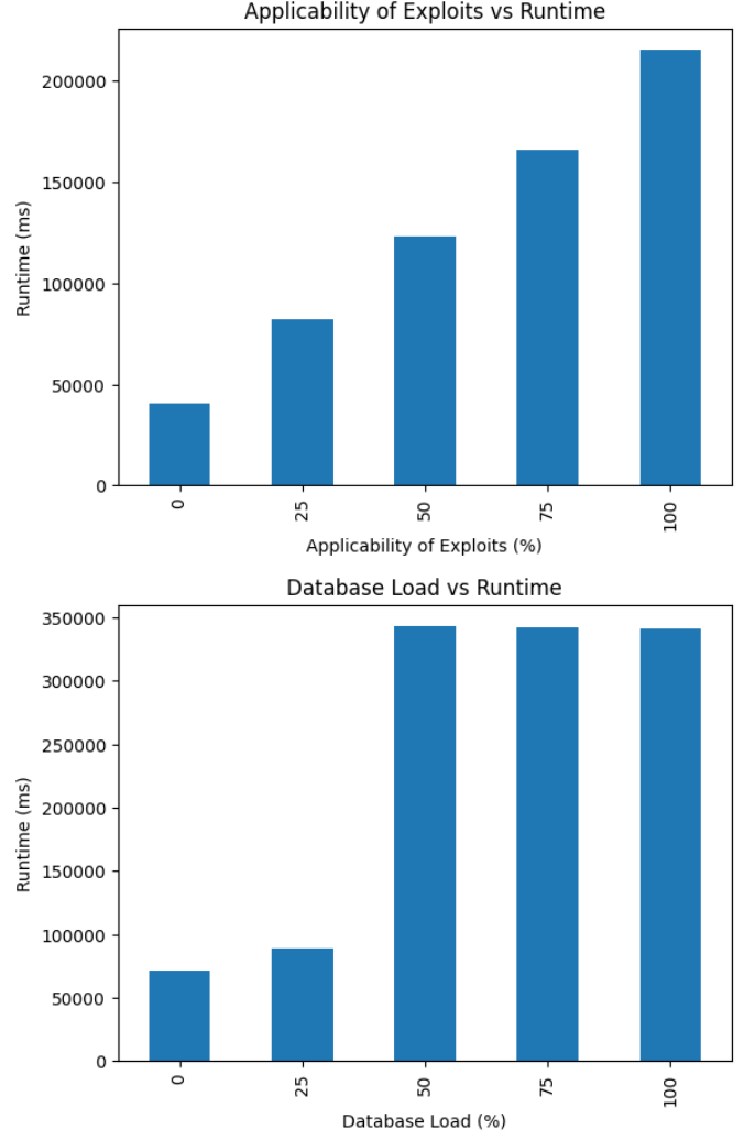
Fig. 10. Applicability of Exploits (%) and Database Load (%) (Averaged) vs. Runtime (ms)
